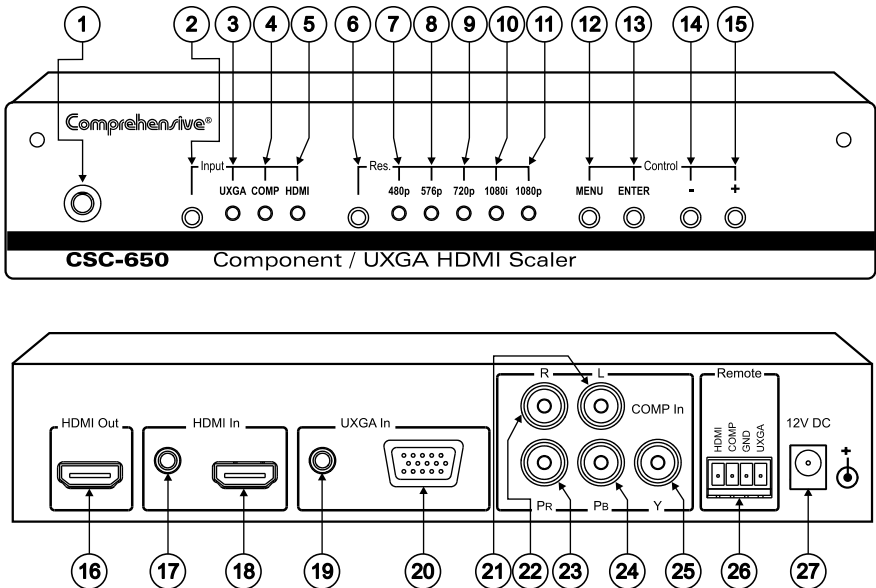
Figure 1: CSC-650 Component / UXGA HDMI Scaler
