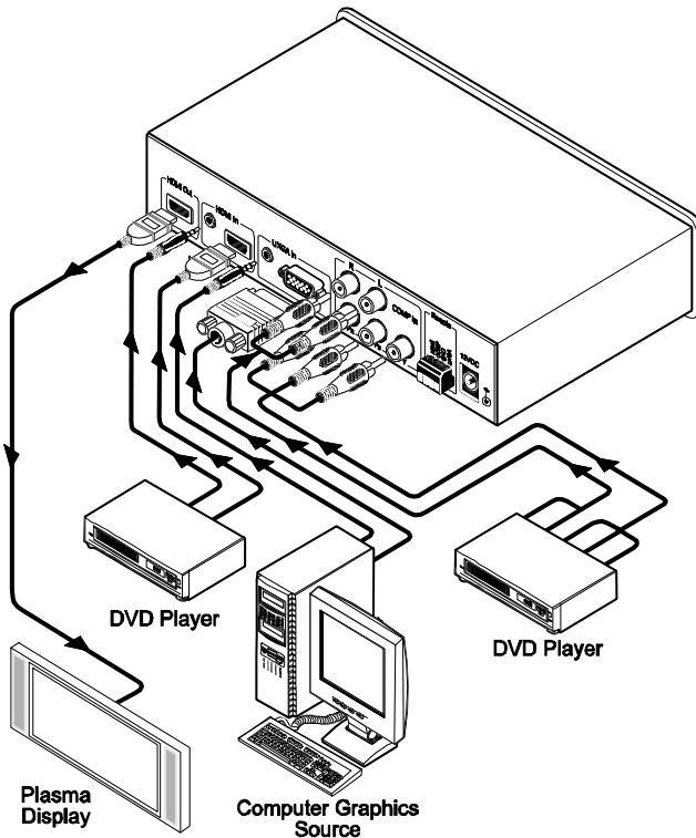
Figure 2: Connecting the CSC-650 Component / UXGA HDMI Scaler
