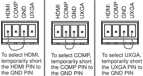
Figure 3: Connecting the Contact Contact Remote Control PINs
